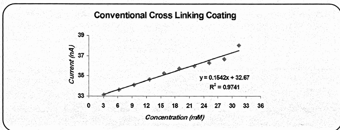
Figure 2. Graph of glucose concentration using conventional cross linking method.
