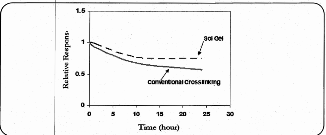
Figure 8. Graphs which show the relative response of sol gel coating and conventional cross linking coating throughout 24 hours of the biosensor in 20 mM glucose concentration.
